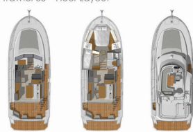
Swift Trawler 35 – Floor Layout
