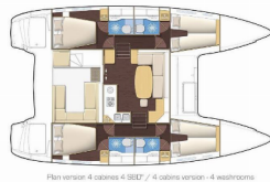
Plan version 4 cabines 4 SBK7 / 4 cabines version - 4 washrooms
